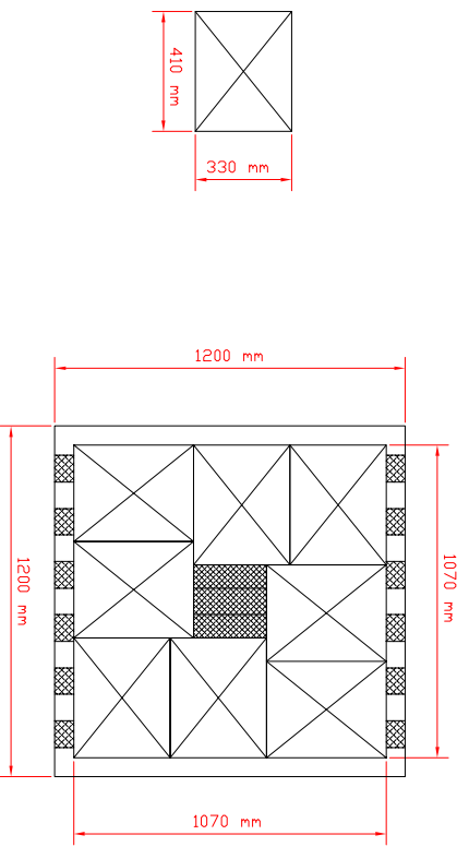
PLANT VIEW
