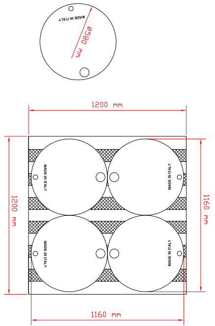
PLANT VIEW
